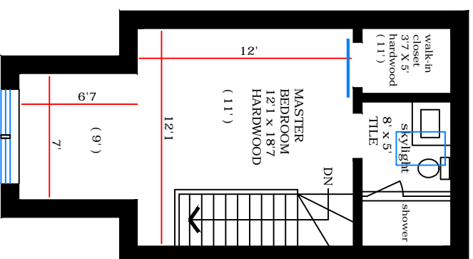
THIRD FLOOR = 300 sq ft
