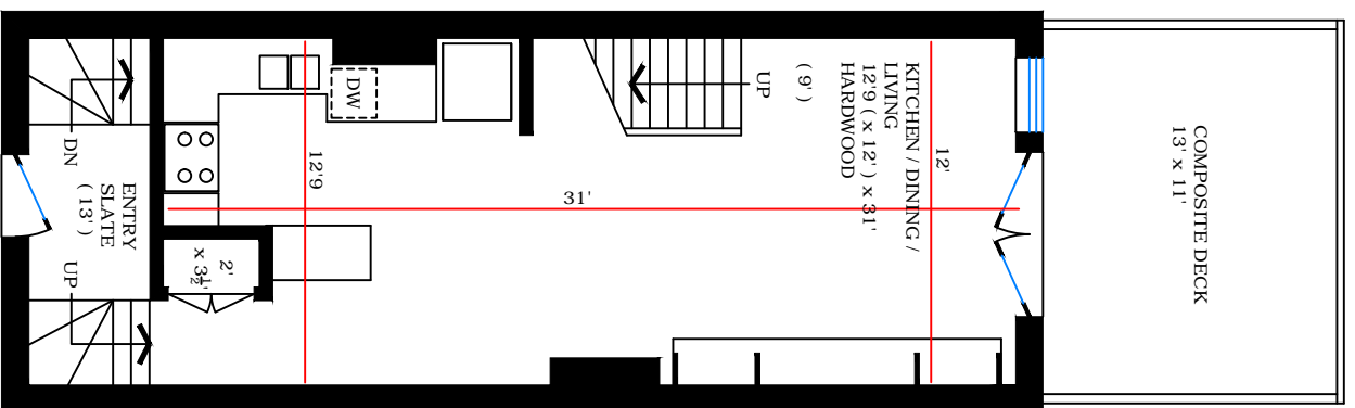
GROUND FLOOR = 520 sq ft
