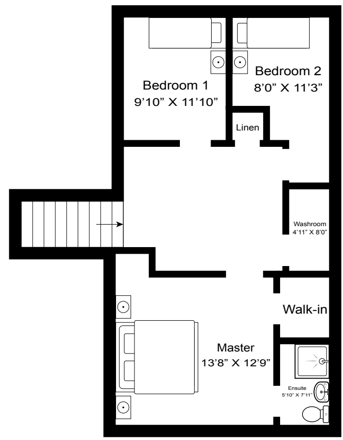
Second Floor
