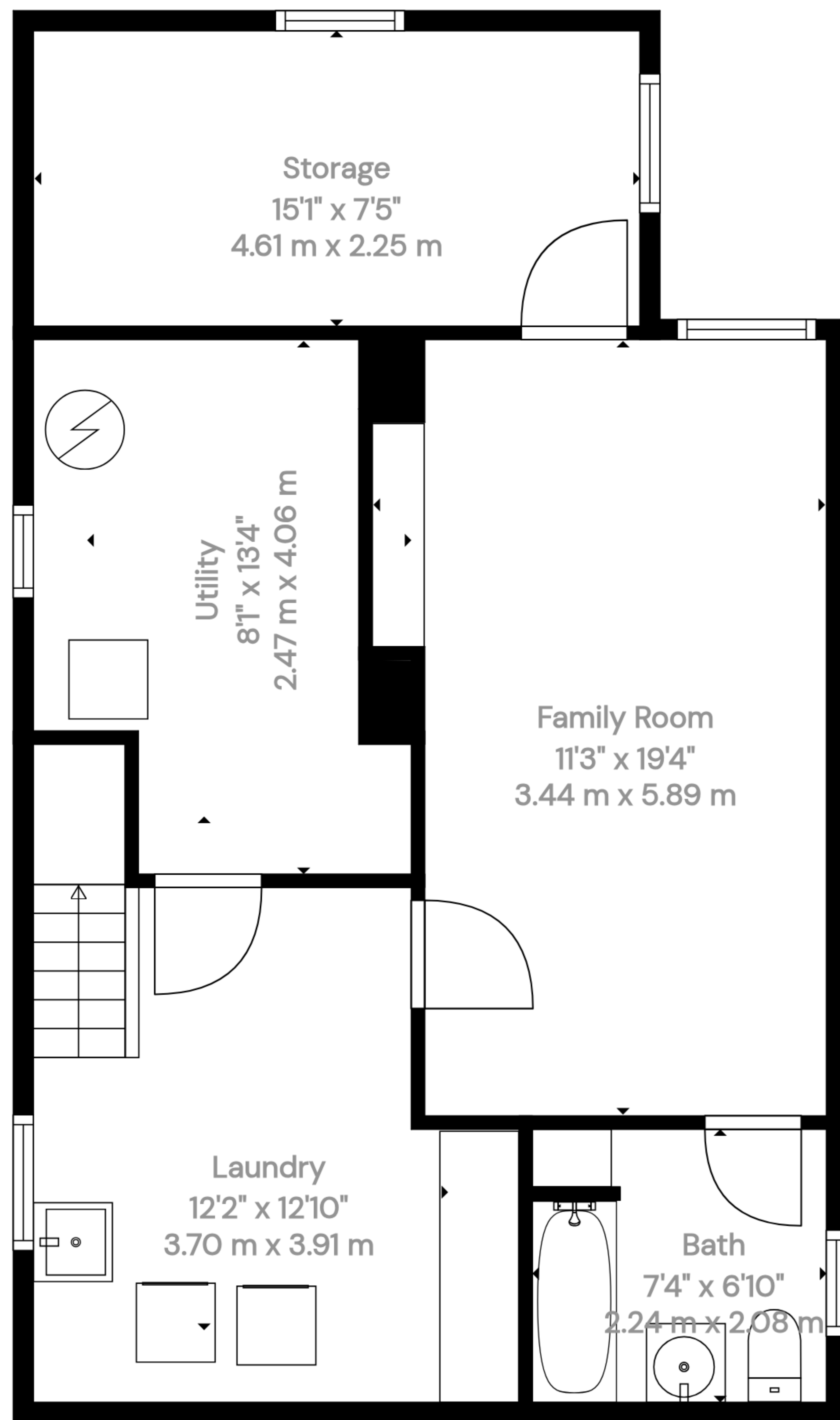
Basement
