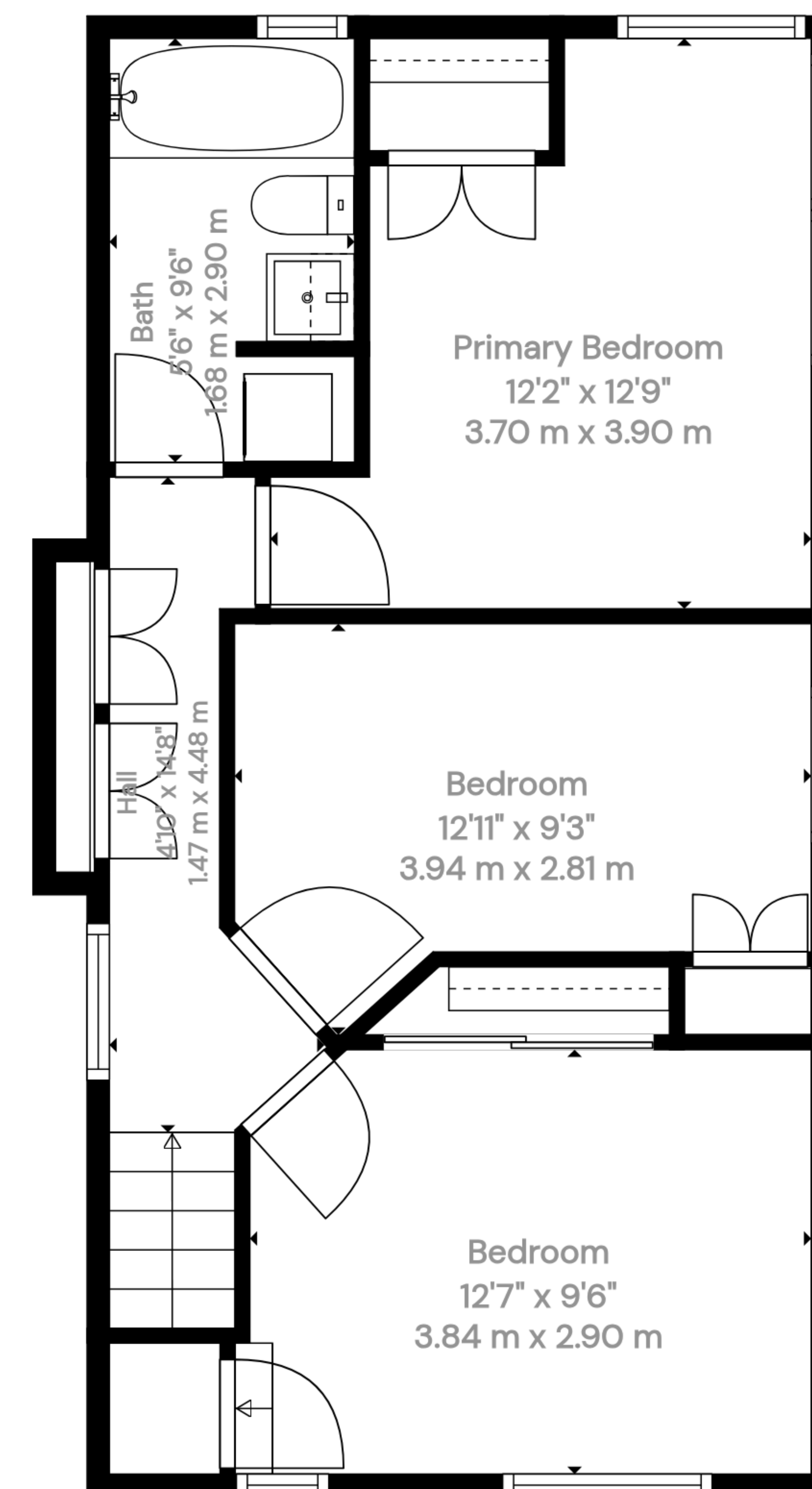
2nd Floor
